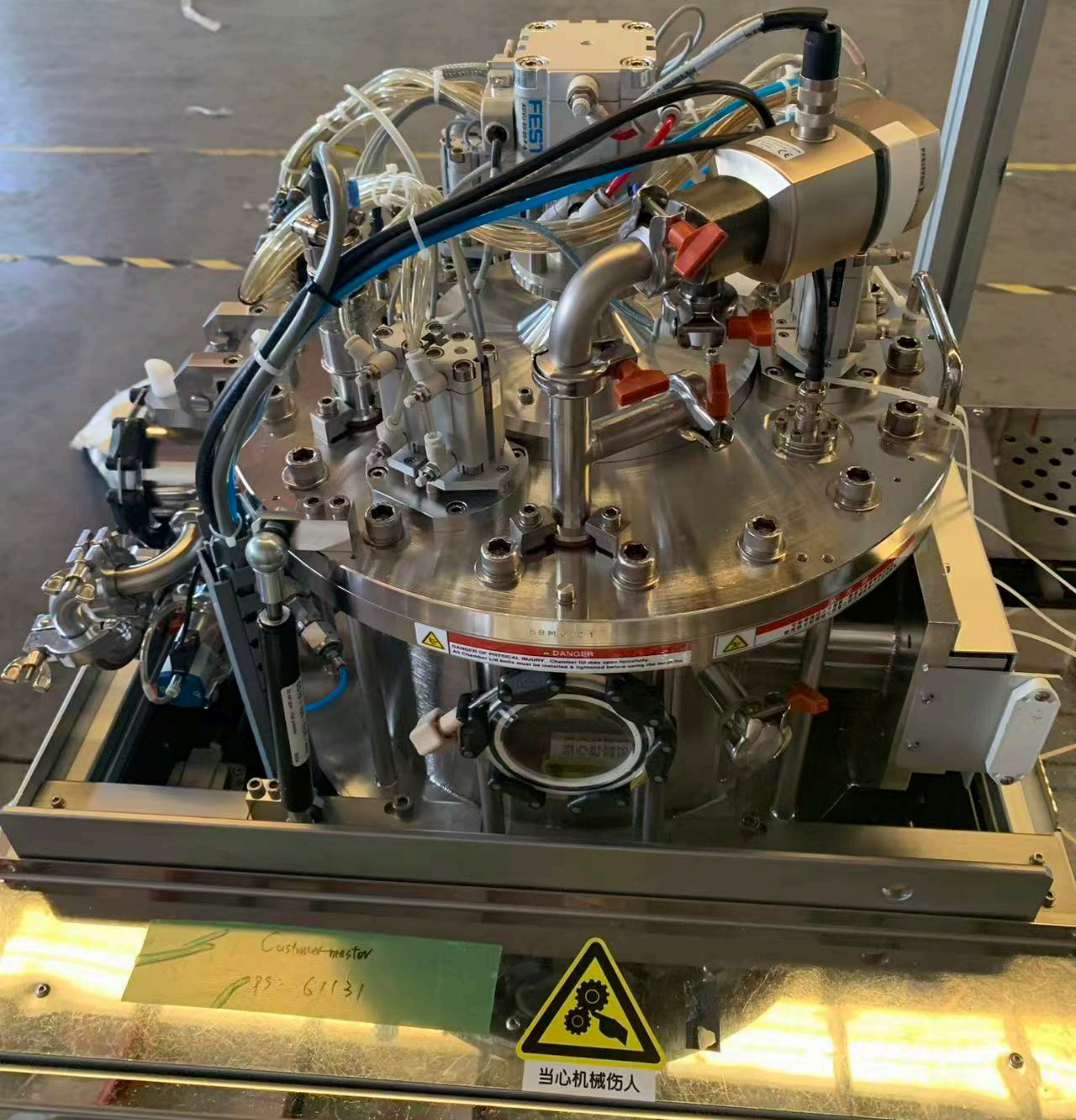
SUSS SB8E Bonding Semiconductor Equipment. Used Semiconductor Equipment
